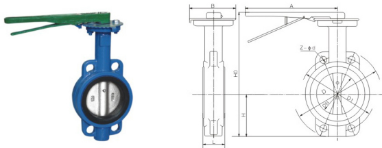
D71 \frac{XA}{A} -10 连接尺寸 Series connection dimensions
