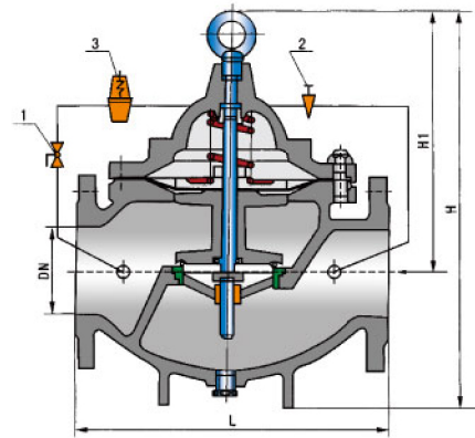
1. Float ball pilot valve 2. ball valve 3. Needle valve
